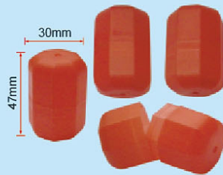
SS2412 30mm x 47mm OCTAGONAL CAPSULE
